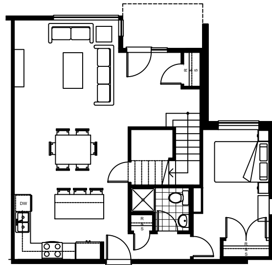
level 1
